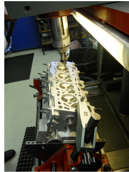
DOHC Cylinder Head Getting Machined for New Valves
